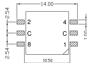
Solder pad layout as viewed from the top of the switch
