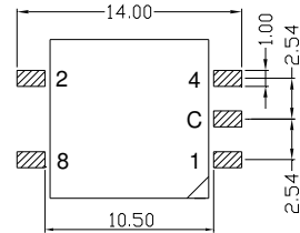
Solder pad layout as viewed from the top of the switch
