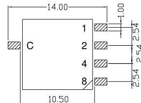
Solder pad layout as viewed from the top of the switch
